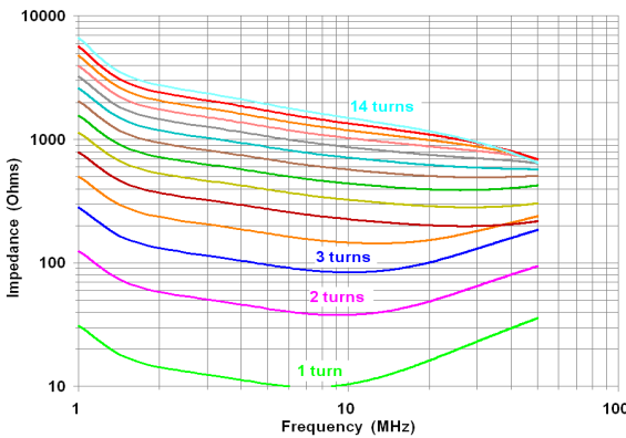
#77 Impedance
