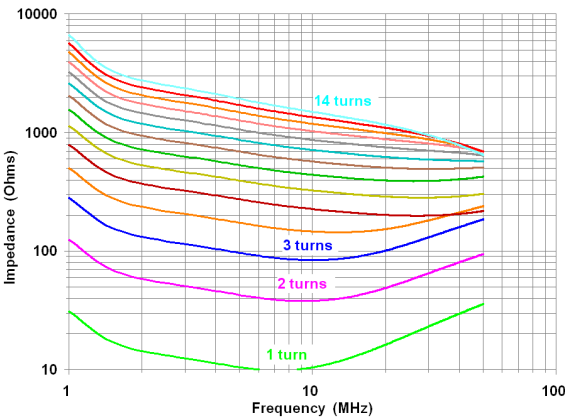
#77 Impedance
