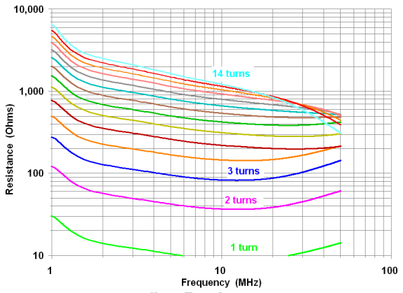
#77 Resistance
