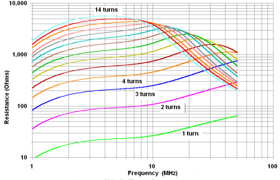
#31 Resistance
