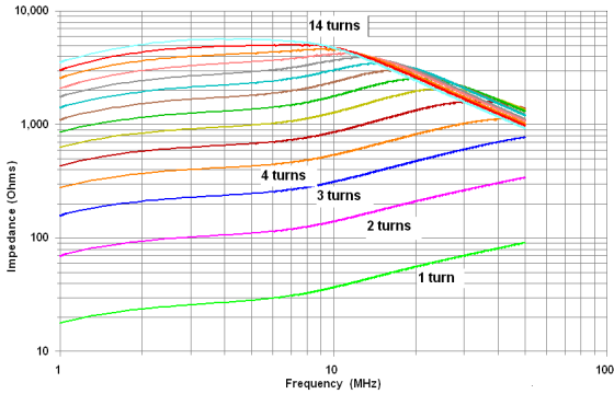
#31 Impedance
