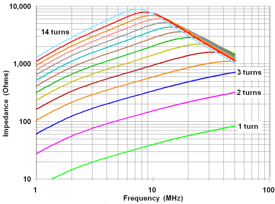
#43 Impedance
