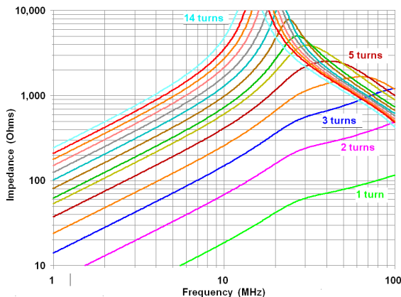
#61 Impedance
