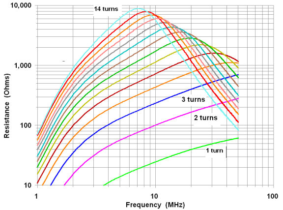
#43 Resistance
