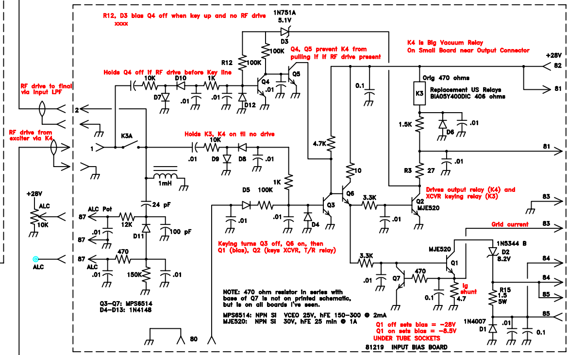
TenTec Titan 425 Power Amp Drawn by K9YC 12Feb08
